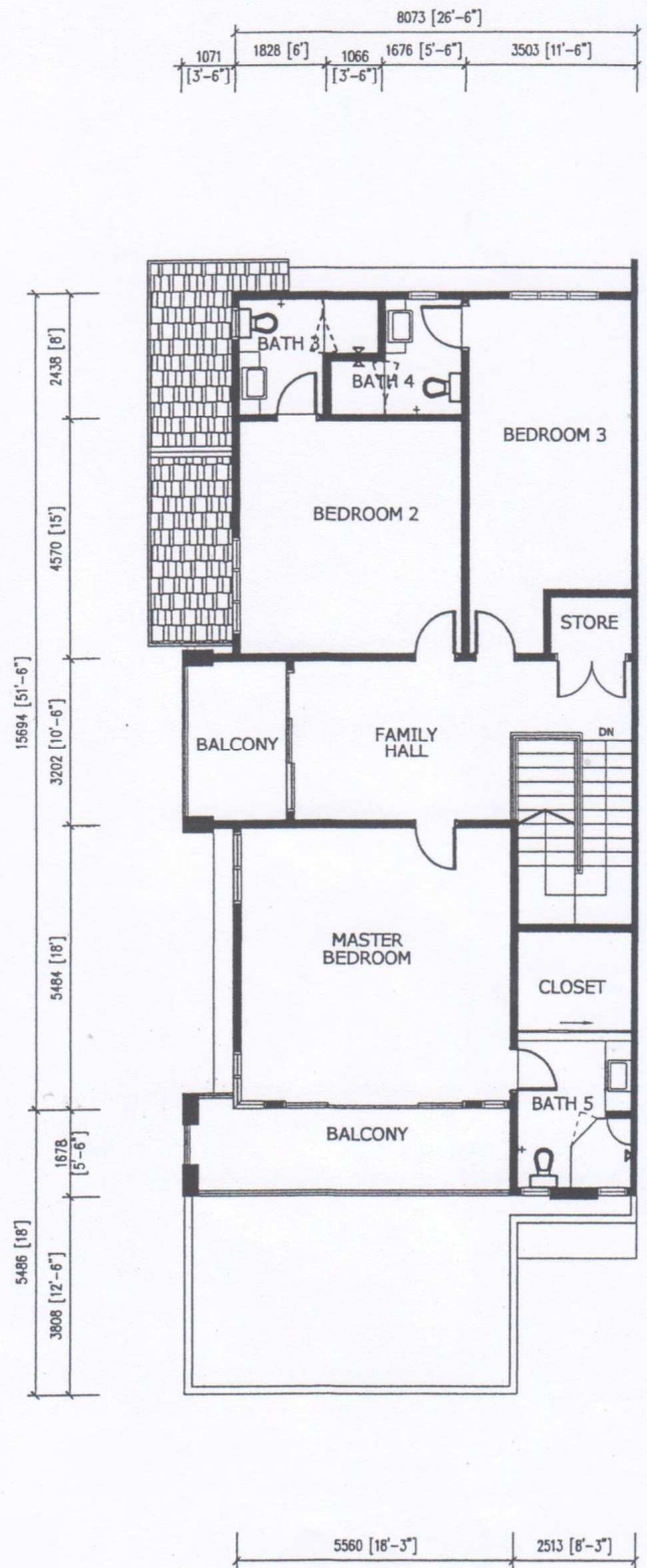
TYPICAL FIRST FLOOR PLAN
